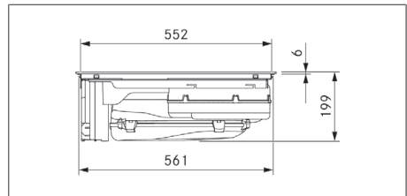
Fig. 3.2 Vista frontal PURSA2/R
