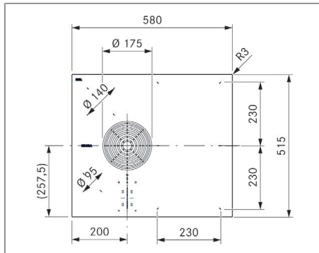
Fig. 3.4 Vista superior PURSU2/R
