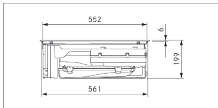
Fig. 3.5 Vista frontal PURSU2/R
