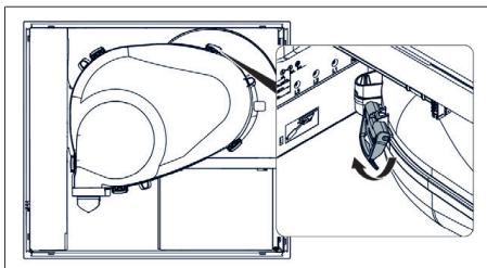
Sl. 11.27 Zapora sesalne enote
